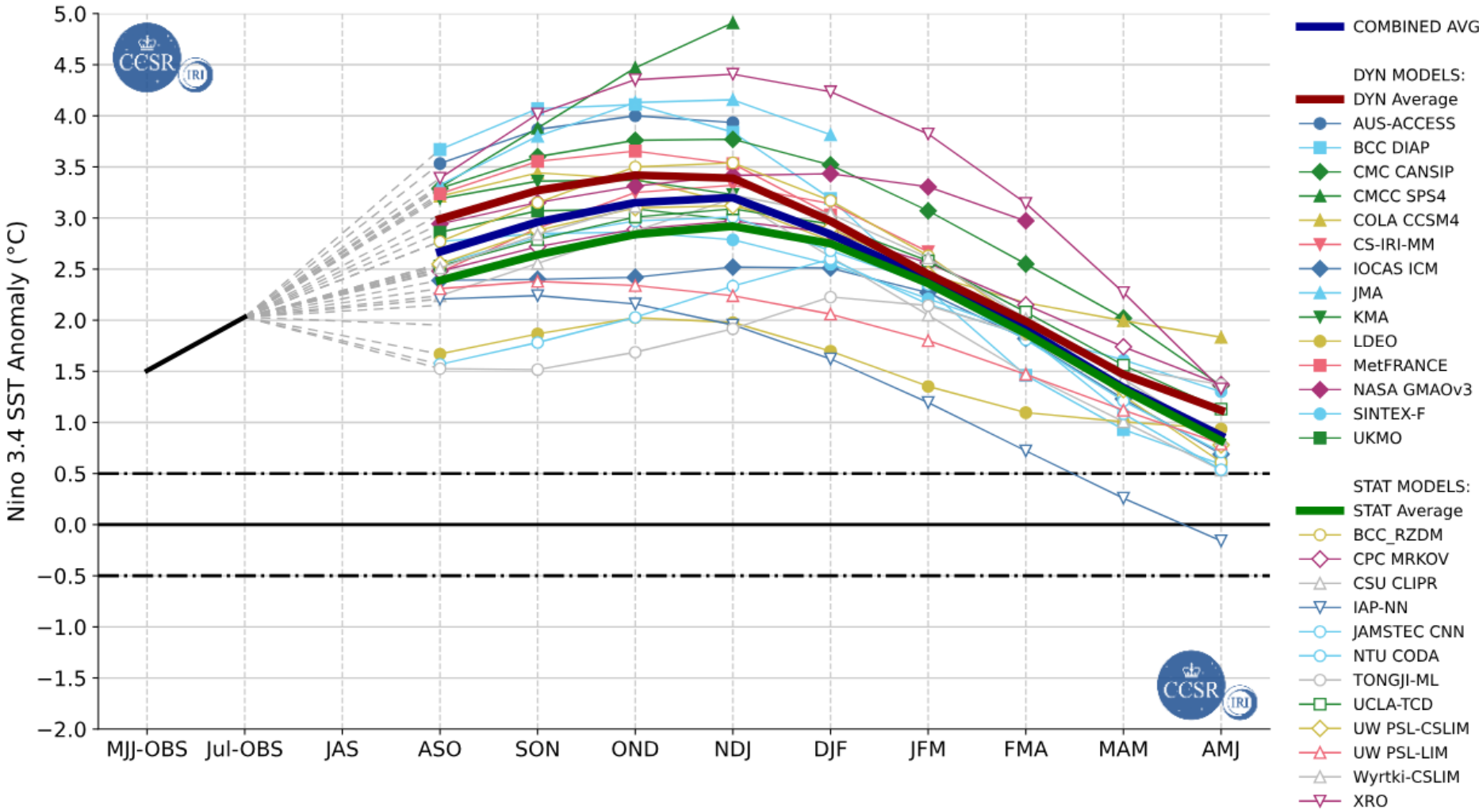
CCSR/IRI Model Predictions of ENSO from Aug 2026
