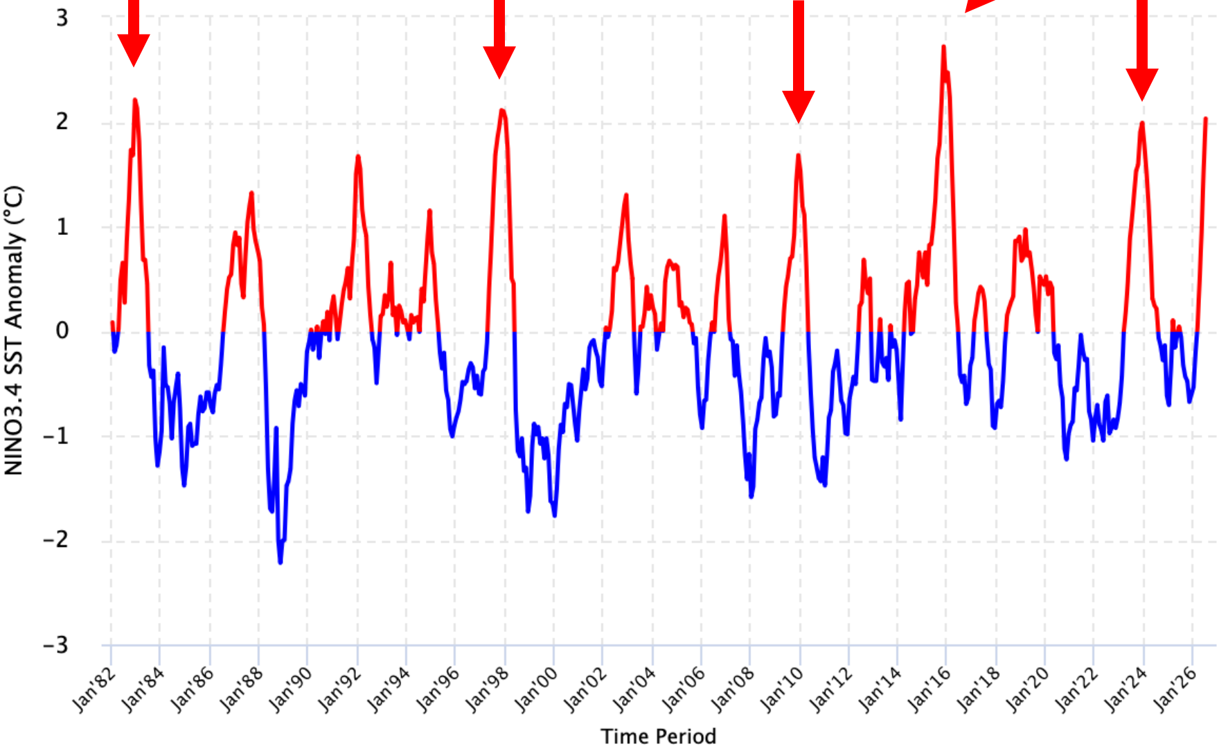
Historical Nino 3.4 Sea Surface Temperature Anomaly
